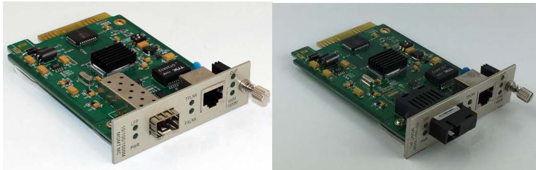
Card with SFP slot(AZ03-1000M-SFP-C) Card with fixed fiber port(AZ03-GSFP-Card)
